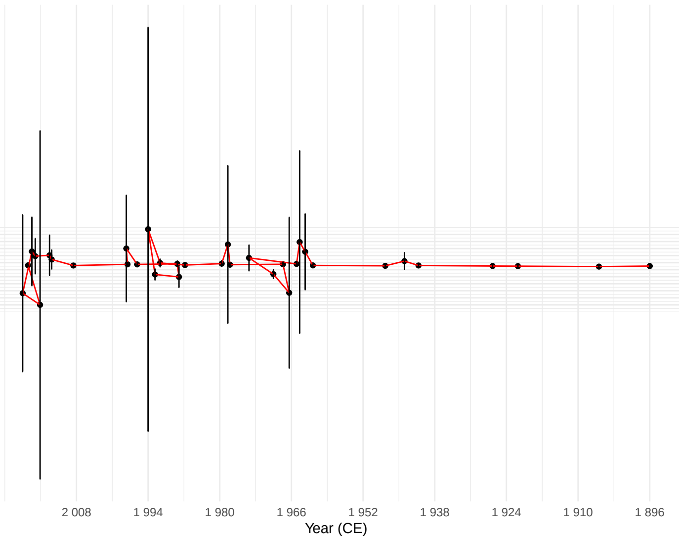
Mass Accumulation Rate by Year
